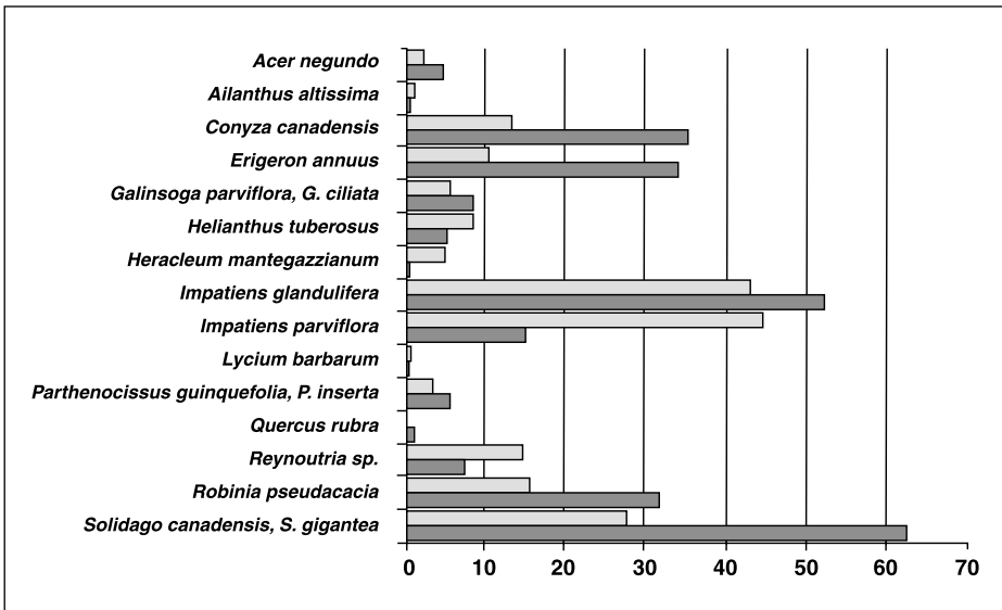
Fig. 1: The share of segments with the presence of each taxons (grey = average of all mapped water courses, black = the Labe river)
