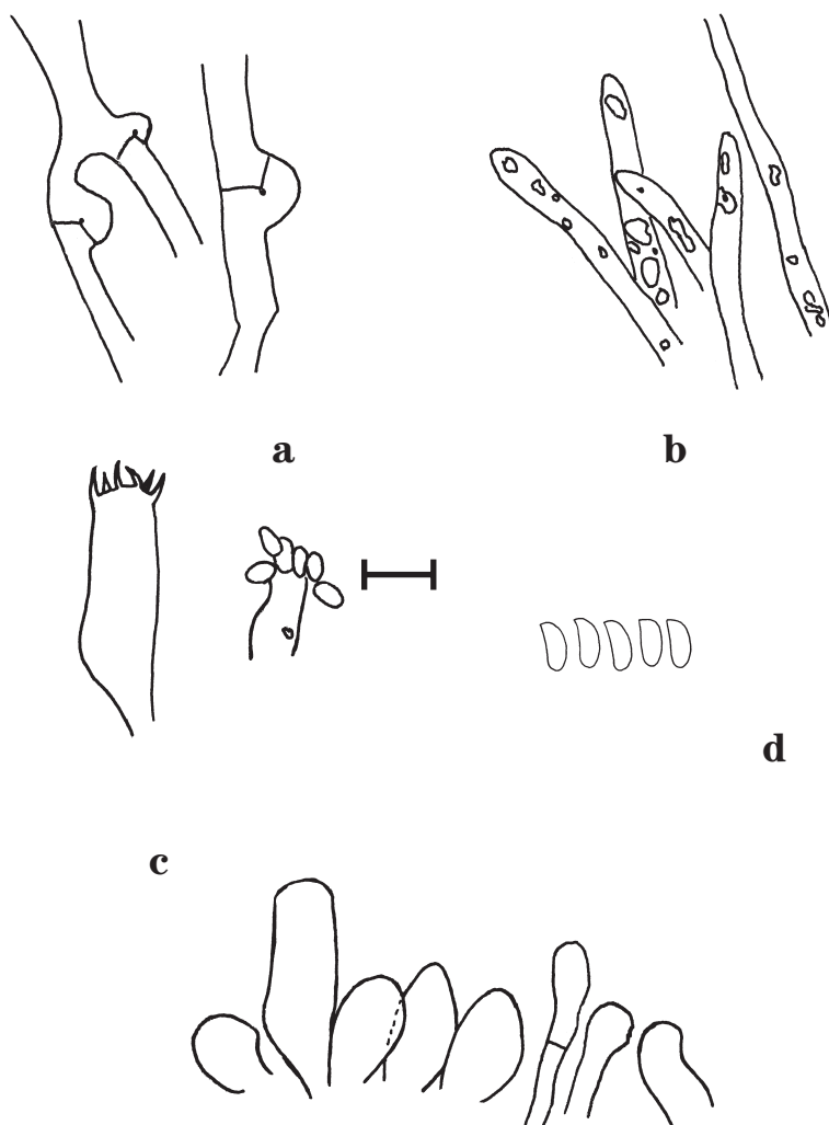
Fig. 1. Sistotrema dennishii : a – clamped hyphae; b – hyphae with oily inclusions; c – basidia; d – spores; e – immature basidia from the hymenium. Bar = 5 \mu m.
