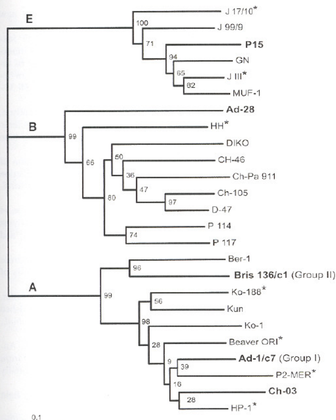
Fig. 2. Phylogenetic tree for 25 isolates of Giardia intestinalis constructed from pooled transformed RAPD data by the Neighbour-Joining method and separated in Assemblages A, B, and E. Branch lengths reflect relative genetic distances between isolates. Bootstrap values for particular branches are indicated. Isolate names printed in bold designate type references for particular genetic assemblages. Asterisks designate isolates in which Giardiovirus dsRNA was detected.
